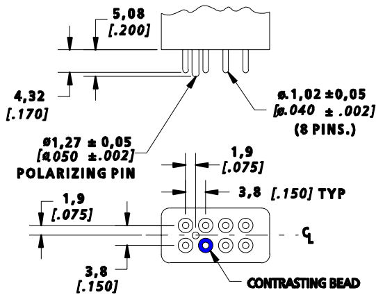
SOLDER PIN
