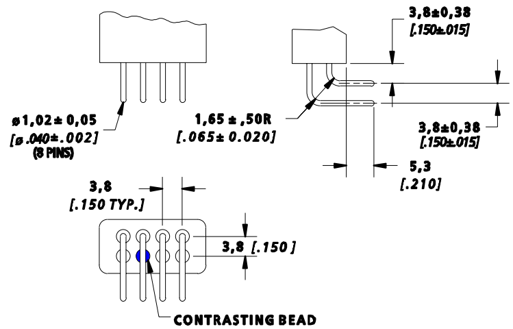
90° SOLDER PIN
